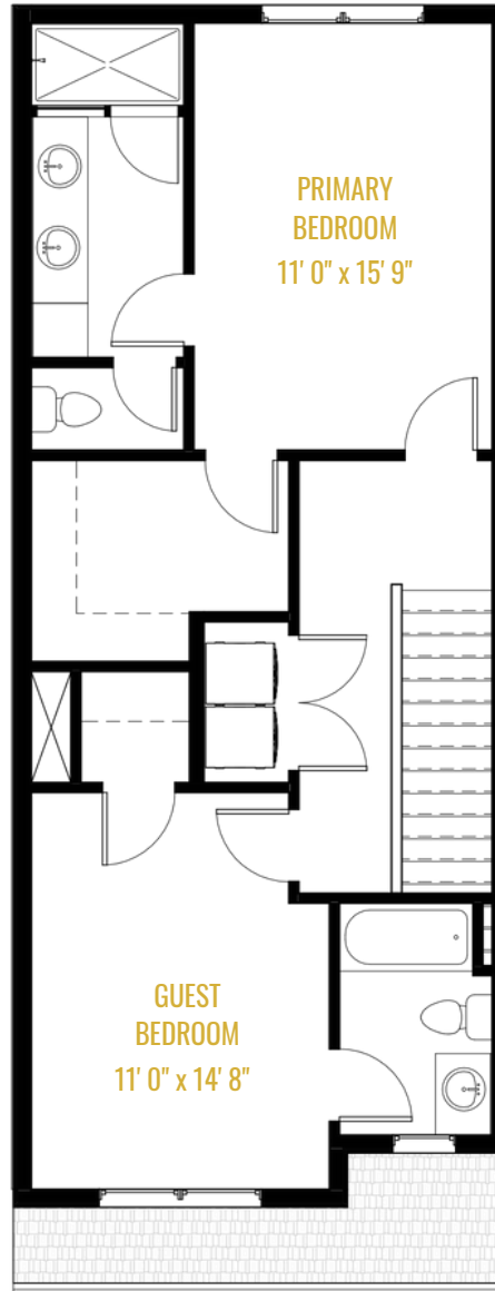
Second Floor
